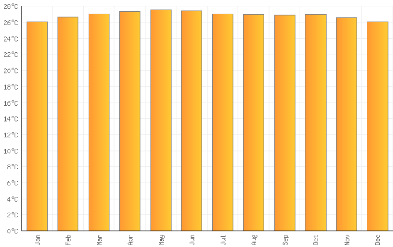
Average monthly temperatures (°C ) in Singapore
