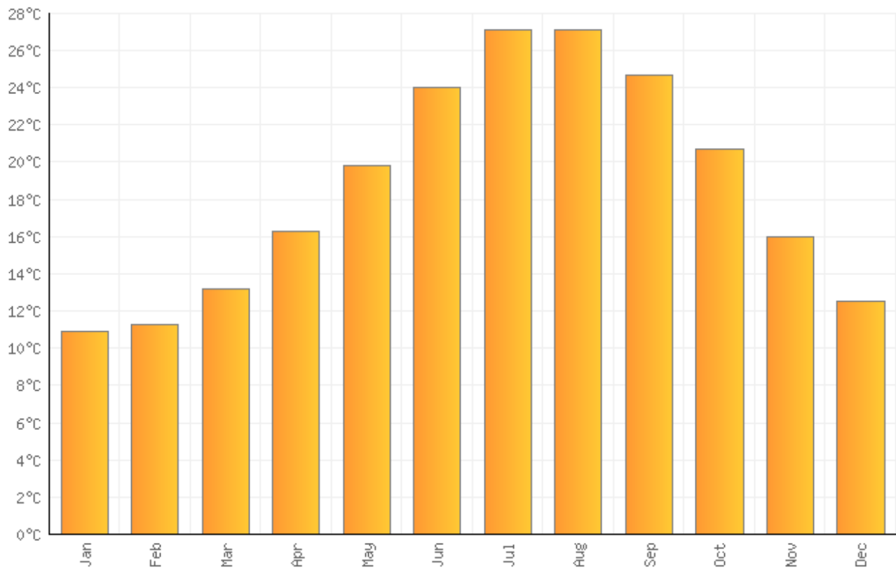
Average monthly temperatures (°C ) in Side
