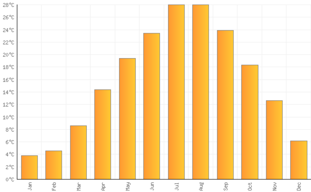
Average monthly temperatures (°C ) in Shanghai
