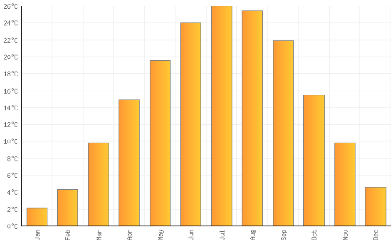
Average monthly temperatures (°C ) in Nashville
