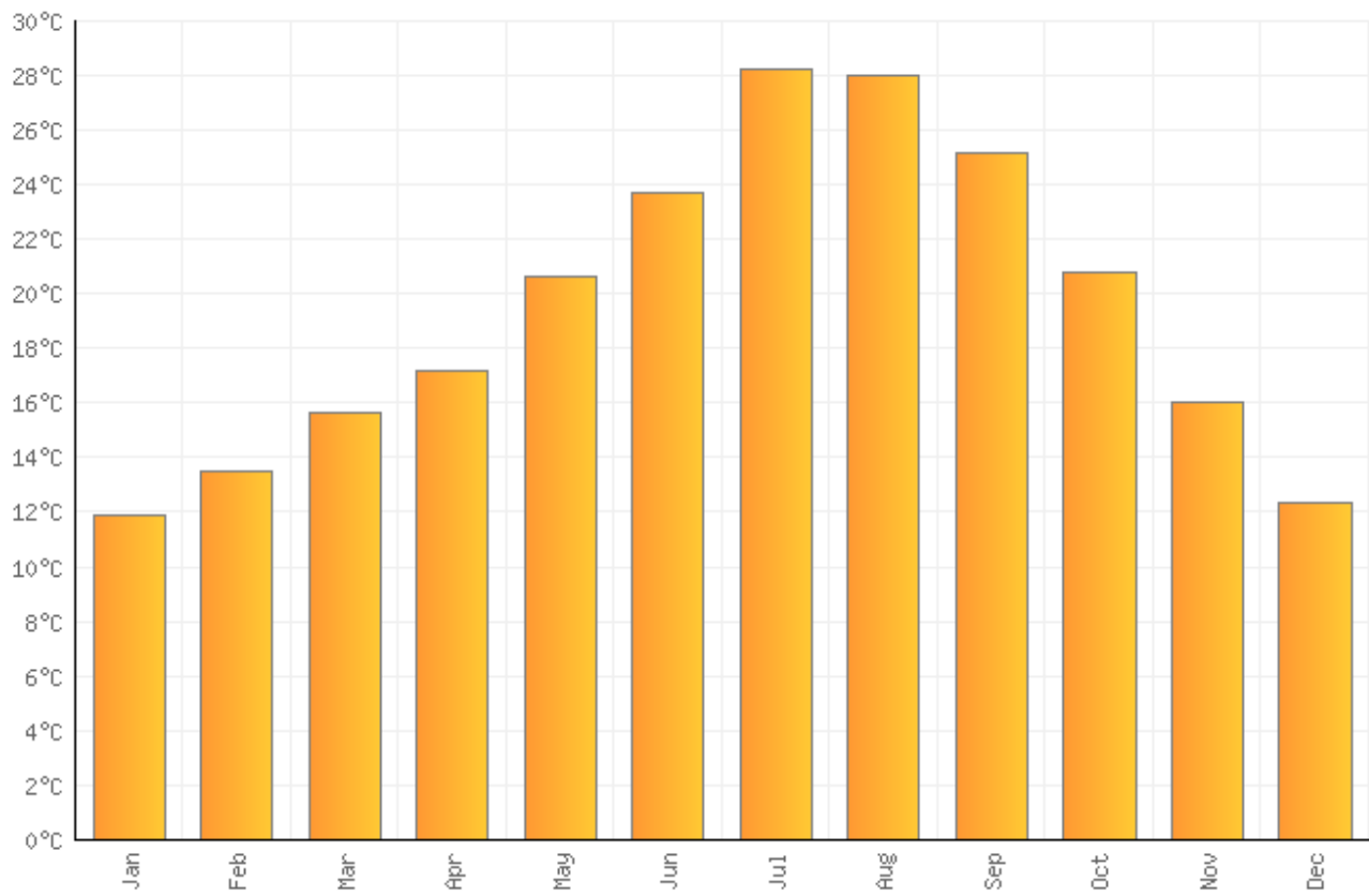
Average monthly temperatures (°C ) in Marrakesh
