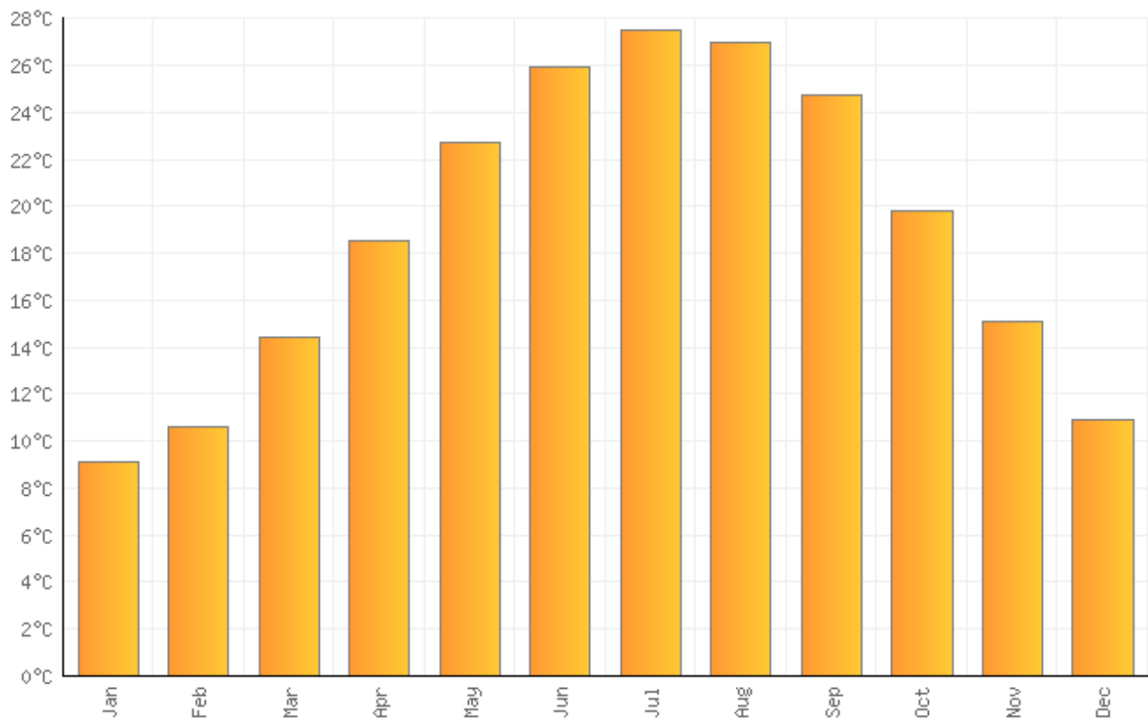
Average monthly temperatures (°C ) in Hilton Head Island
