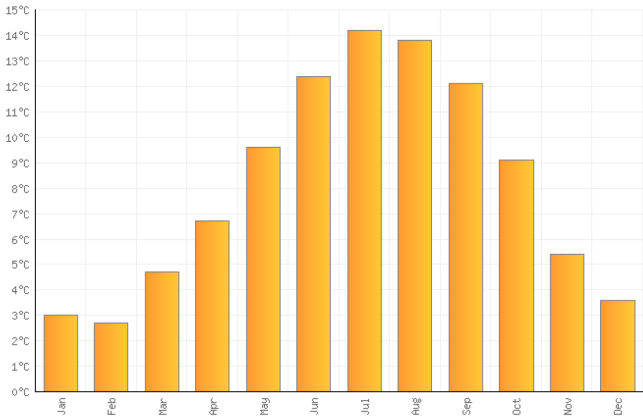
Average monthly temperatures (°C ) in Edinburgh
