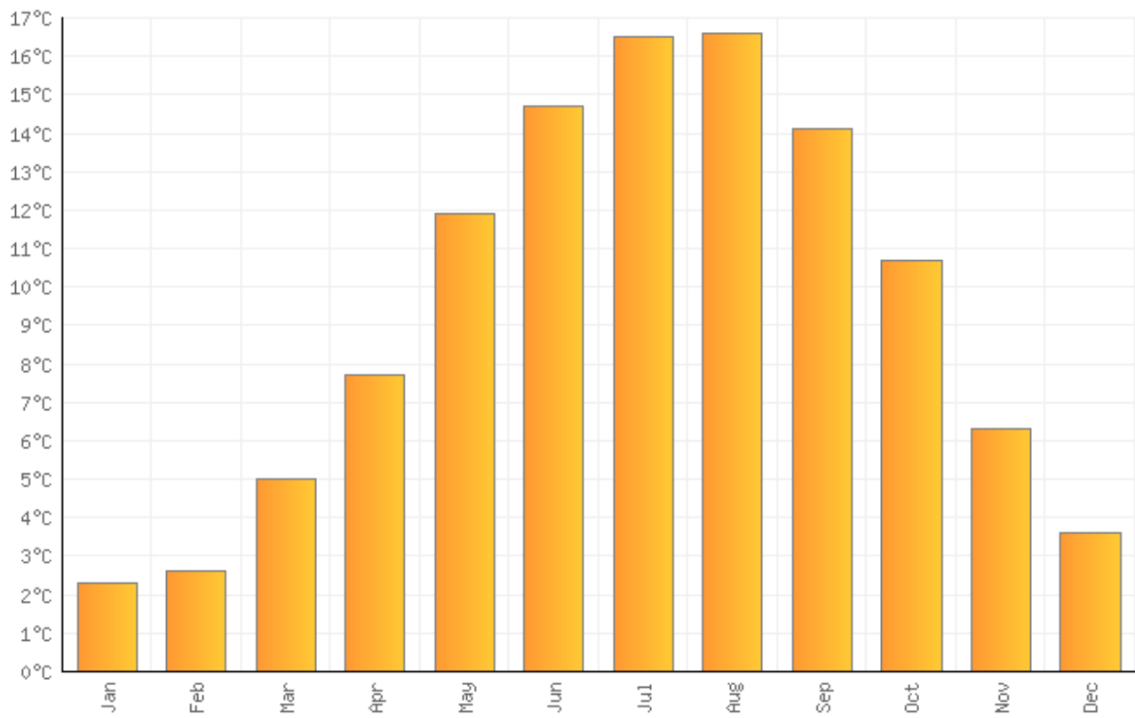
Average monthly temperatures (°C ) in Amsterdam
