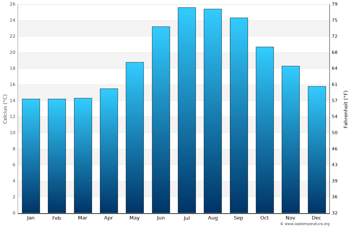
Dubrovnik water temperature
