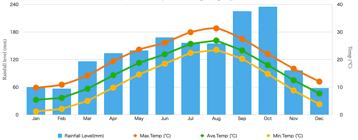
Rainfall Level & Average Temperature in Tokyo (1991-2020) (Data source: Japan Meteorological Agency)
