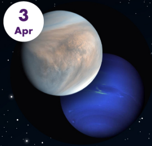
Conjunction of Venus and Neptune
